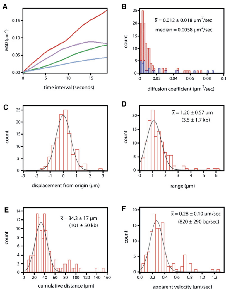
Figure 4. General Characteristics of Msh2-Msh6 Diffusion
