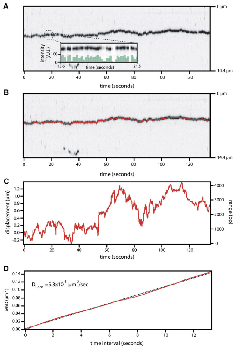
Figure 3. Msh2-Msh6 Moves on DNA via 1D Diffusion
