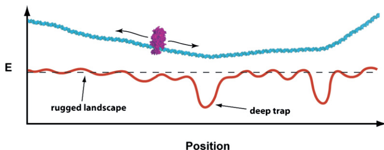
Figure 7. Model for DNA Scanning by Msh2-Msh6
