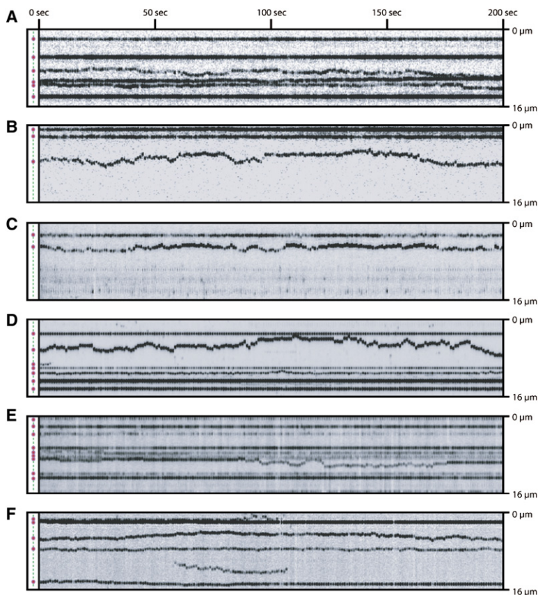
Figure 2. Visualizing Movement of Msh2-Msh6 on DNA
