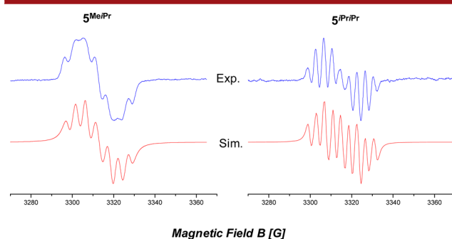
Figure 2. Experimental and simulated EPR spectra of 5^{\text{MeiPr}} and 5^{\text{iPrPr}} in THF.
