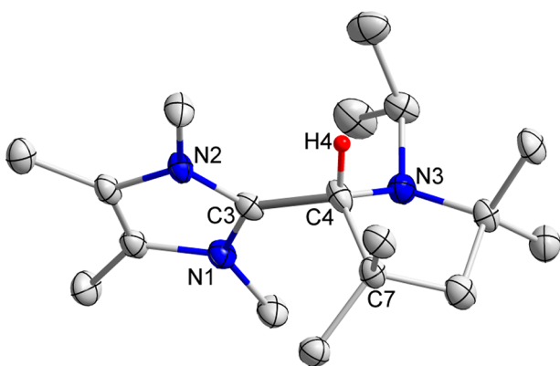
Figure 1. Molecular structure of 3^{\text{MeiPr}} in the solid state (thermal ellipsoids at 50%, triflate anion, and H atoms except C4–H omitted for clarity). Selected bond lengths (Å) and angles ( ^\circ ): C3–C4 1.517(3); N2–C3–N1 107.2(2), N3–C4–C7 105.8(2).
