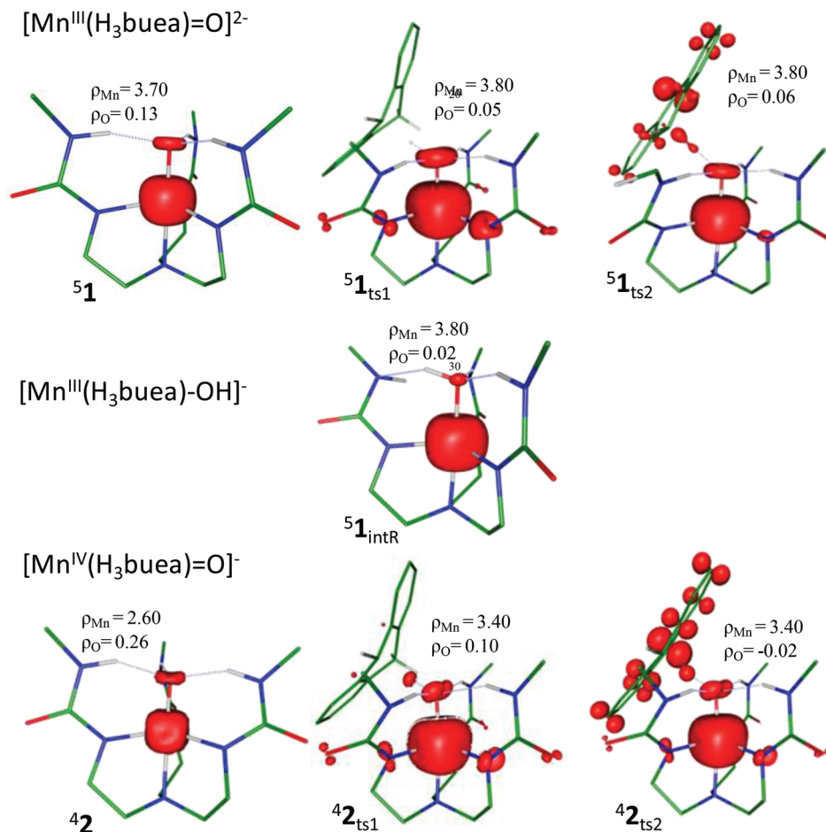
Fig. 4 Computed spin density plots for ts1, ts2 and ^5\mathbf{1}_{\text{intr}} of species 1 and 2 .
