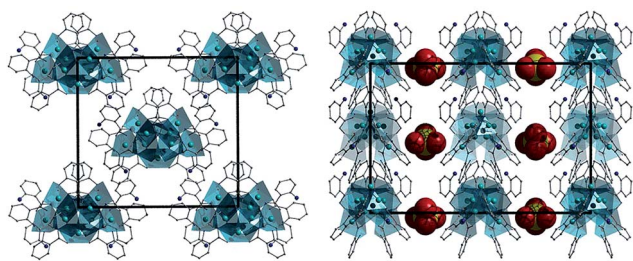
Fig. 5 Crystal packing observed in 4 as viewed along the a (left) and b (right) cell direction. All hydrogen atoms and solvents of crystallisation have been omitted for clarity. The \text{SO}_4^- counter anions are represented as space-fill in the figure on the right and removed for clarity on the left.
