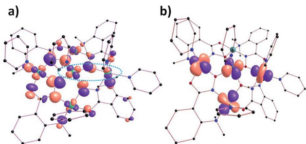
Fig. 12 (a) One of the MOs of complex 2 highlighting orthogonality between the d_{x^2-y^2} magnetic orbitals of centres Ni1 and Ni5 respectively (circled). (b) Natural hybrid orbitals 15 representing the dominant orbital interactions in the molecular plane of complex 2 (see ESI Table S4† for computed overlap integral values).
