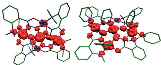
Fig. 11 DFT computed spin density plots for complex 1 (left) and 2 (right). Here red and blue indicates positive and negative spin densities respectively.
