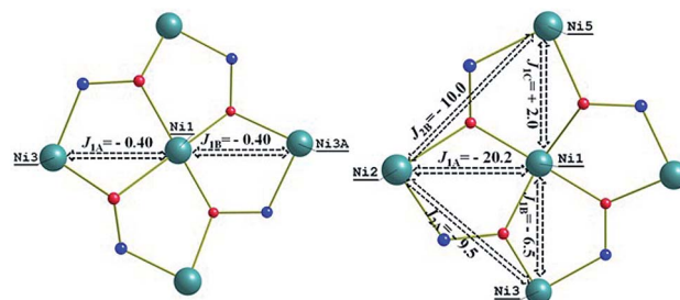
Fig. 10 Schematic representation of the magnetic coupling constants (in \text{cm}^{-1} ) in 1 (left) and 2 (right).
