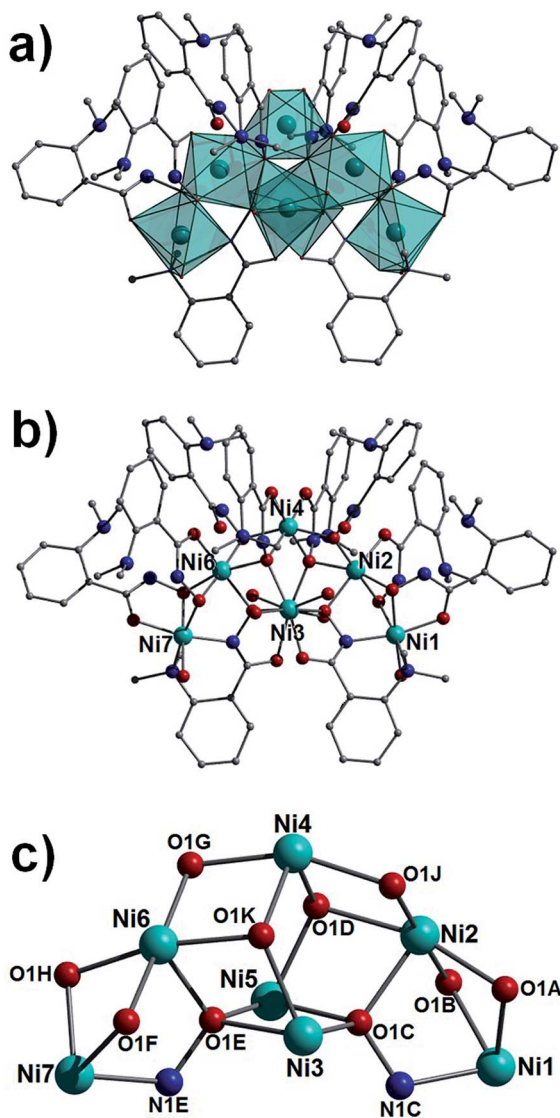
Fig. 3 Polyhedral (a) and regular (b) representation of the crystal structure in 3. (c) Metallic core in 3. Colour code as in Fig. 1. Hydrogen atoms have been omitted for clarity.
