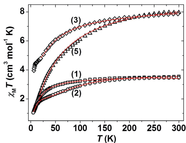
Fig. 7 Plot of \chi_{\text{M}}T vs. T for complexes 1 ( \square ), 2 ( \circ ), 3 ( \diamond ) and 5 ( \triangle ). The solid lines represent best-fits of the experimental data. See text for details.
