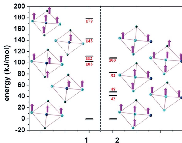
Fig. 6 All possible total spin ( s ) configurations of the individual \text{Ni}(\text{II}) ions in complexes 1 and 2 , with their respective energies ( \text{kJ mol}^{-1} ).
