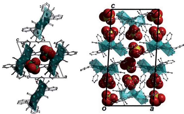
Fig. 2 Packing arrangements of 1 (left) and 2 (right) as viewed down the b axis of their respective unit cells. Hydrogen atoms have been omitted for clarity. Perchlorate counter anions are represented in the space-fill mode.
