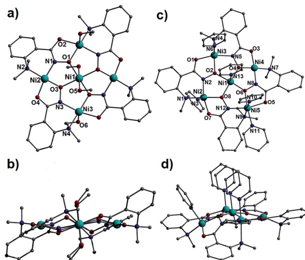
Fig. 1 Crystal structures of 1 and 2 viewed perpendicular (a and c) and parallel (b and d) to their \{Ni(II)_5\} planar cores. Colour code: light blue (Ni), red (O), dark blue (N), grey (C). The perchlorate counter anions have been omitted for clarity. Hydrogen atoms have been omitted for clarity in all cases.
