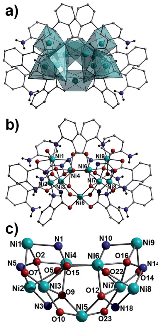
Fig. 4 Polyhedral (a) and regular (b) representation of the crystal structure in 5. (c) The metallic core in 5. Colour code as used in Fig. 1 and elsewhere in the text. The majority of H atoms have been omitted for clarity however the -\text{NH}_2 protons are represented as black spheres.
