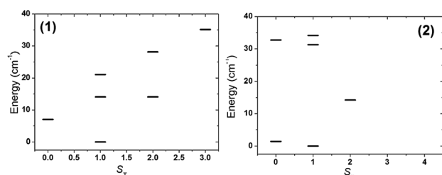
Fig. 9 Energy versus total spin state for the lowest lying S states in 1 and 2 as determined from the isotropic fit of the susceptibility data.
